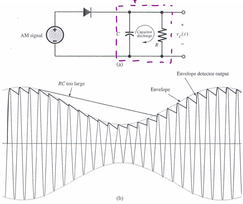
Figure 25: Envelope detector for AM [5, Fig. 4.11].
