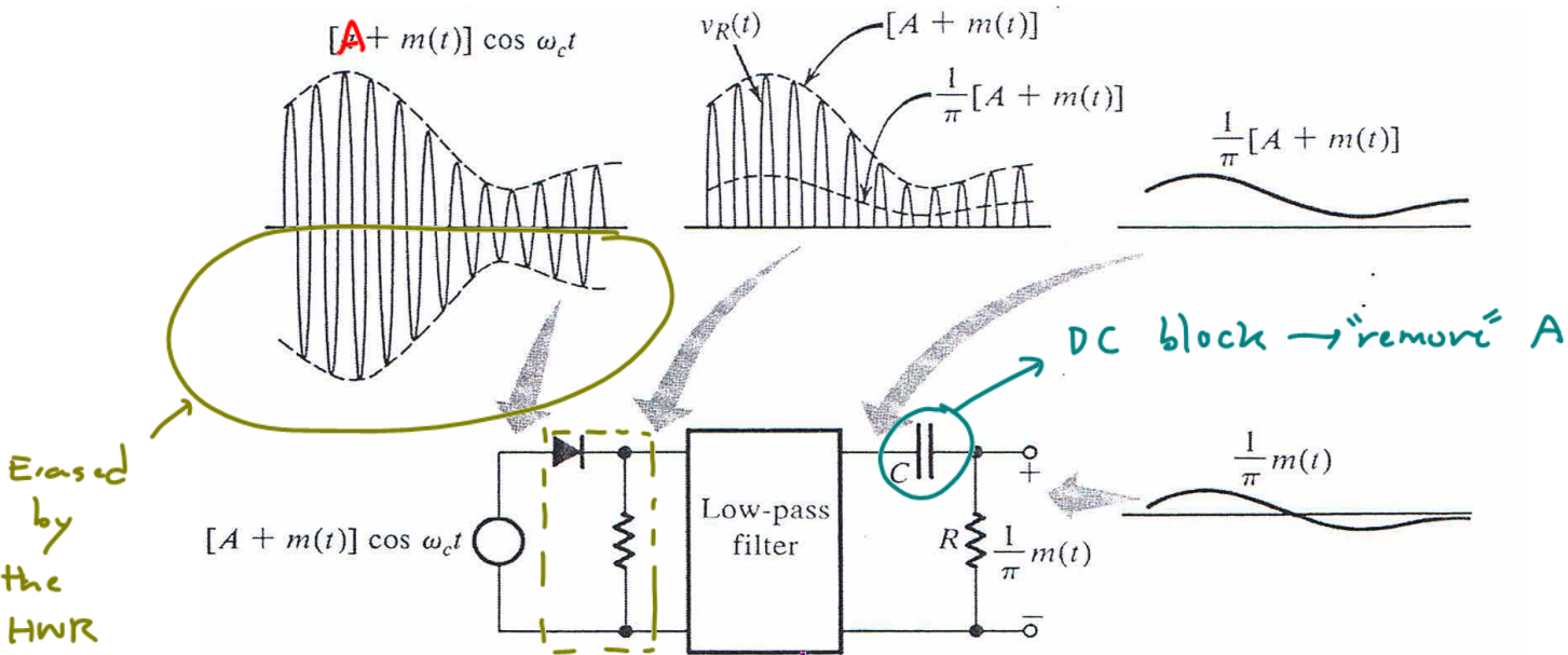
Figure 24: Rectifier detector for AM [5, Fig. 4.10].
