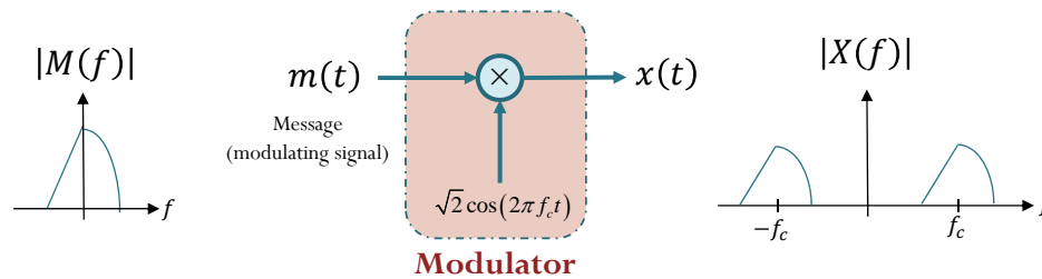
Figure 21: DSB-SC modulation.
