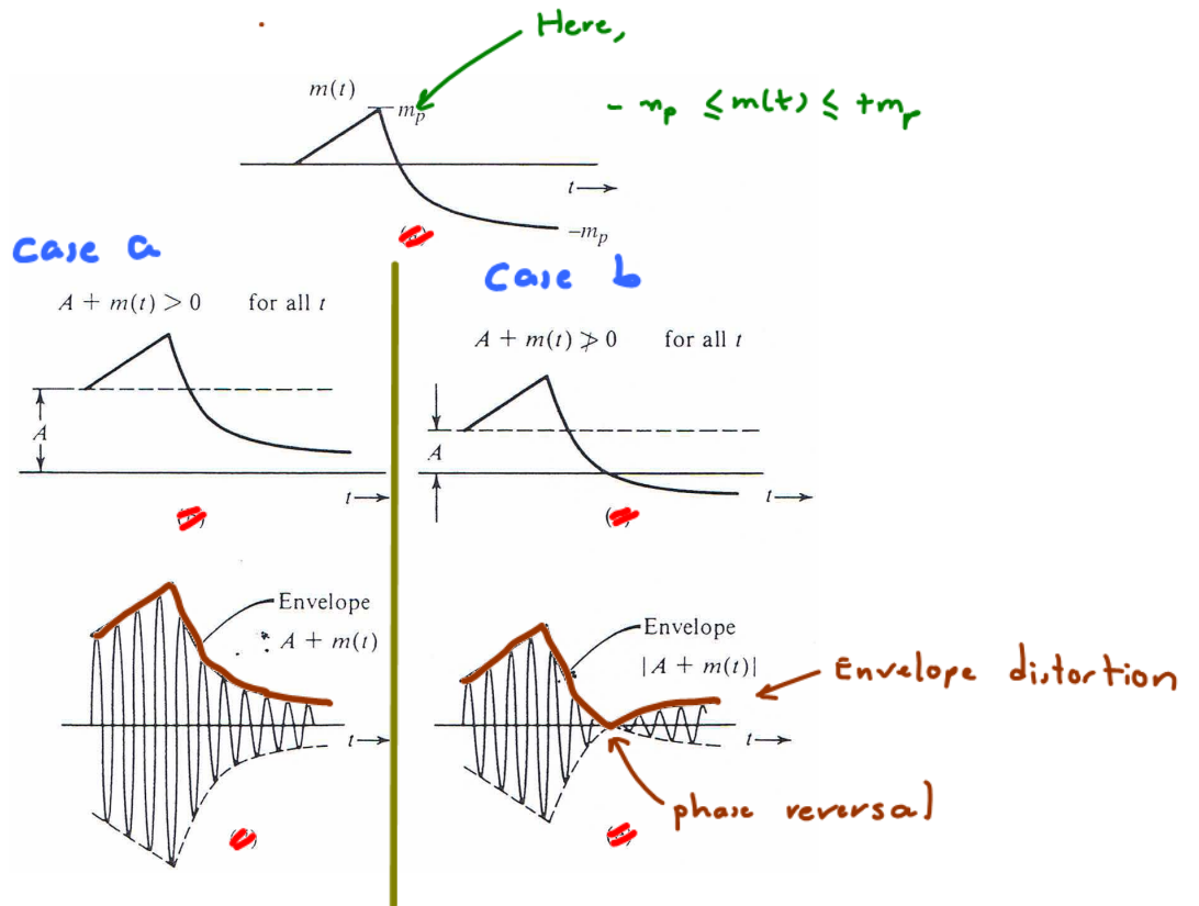
Figure 22: AM signal and its envelope [5, Fig 4.8]
