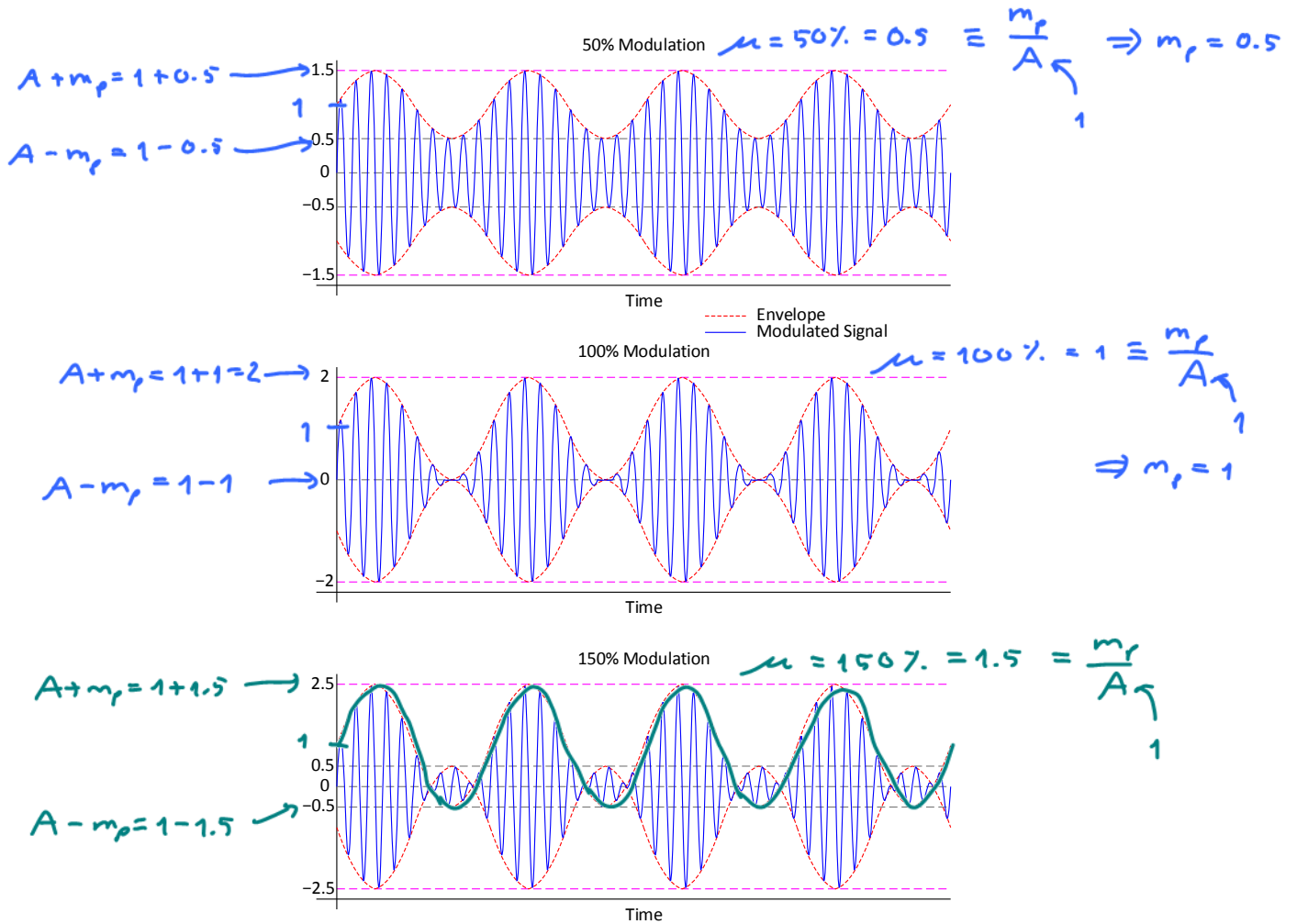
Figure 23: Modulated signal in standard AM with sinusoidal message
